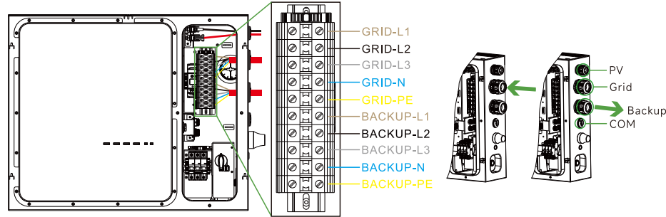
Terminal Layout
