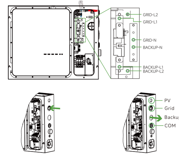
Terminal Layout
