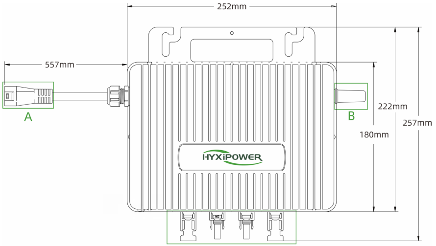
A: AC Branch Connector B: Antenna C: DC terminal
