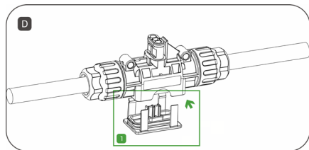
Insert the lower T-junction cover back into place and make sure it is secure.
